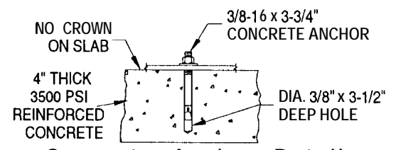
Concrete Anchor Detail
