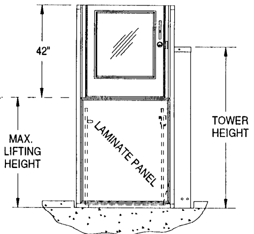
Upper Landing Side Elevation
