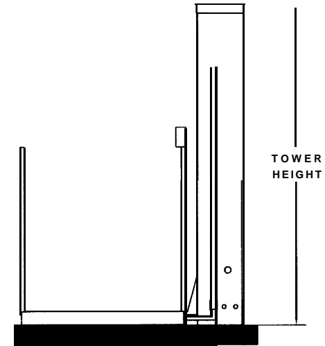
LOWER LANDING SIDE ELEVATION
