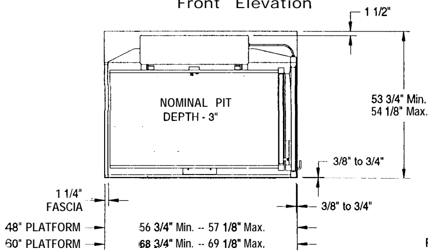
Pit Layout (Ref. ASME A17.1 Part XX)
